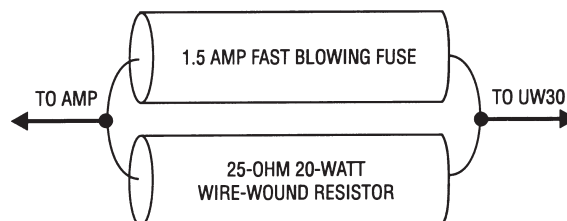
Figure 2 Fuse Recommendation
