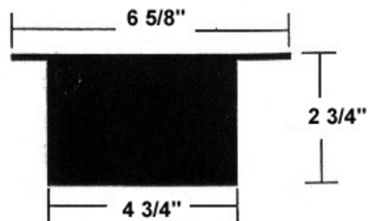
SIDE VIEW BOX
