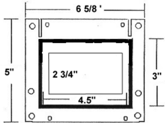
TOP VIEW BOX
