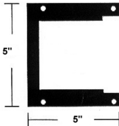
TOP VIEW SPACER
