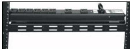
PB-XS mounts PD-815SC and PD-815SC-NS power strips between rackrail
