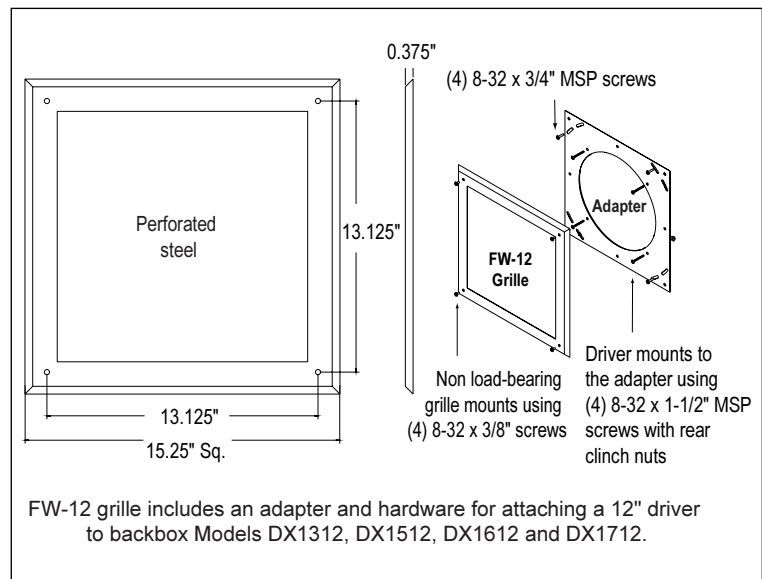
FW-12 Grille for mounting a 12" speaker to DX Series 12" backboxes
