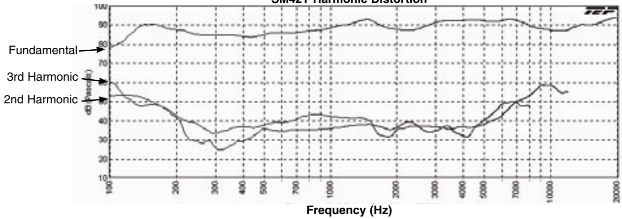
SM42T Harmonic Distortion
