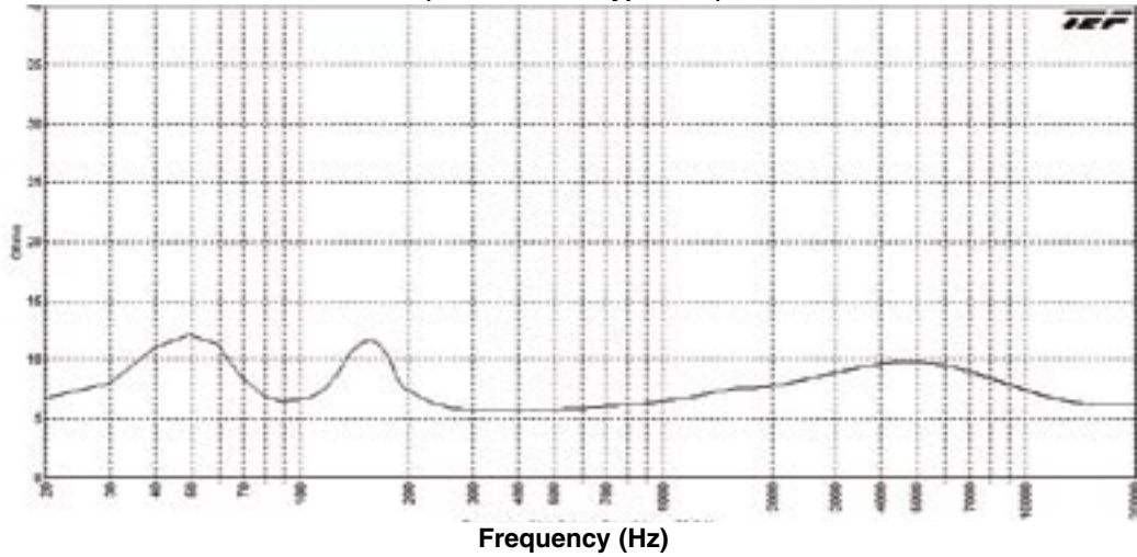
SM42T Impedance (ohms) vs. Frequency (Transformer Bypassed)
