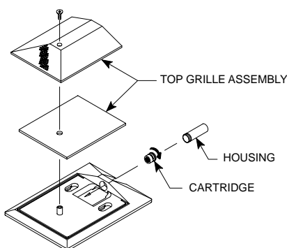
BETA 91 MICROPHONE AND CARTRIDGE FIGURE 2
