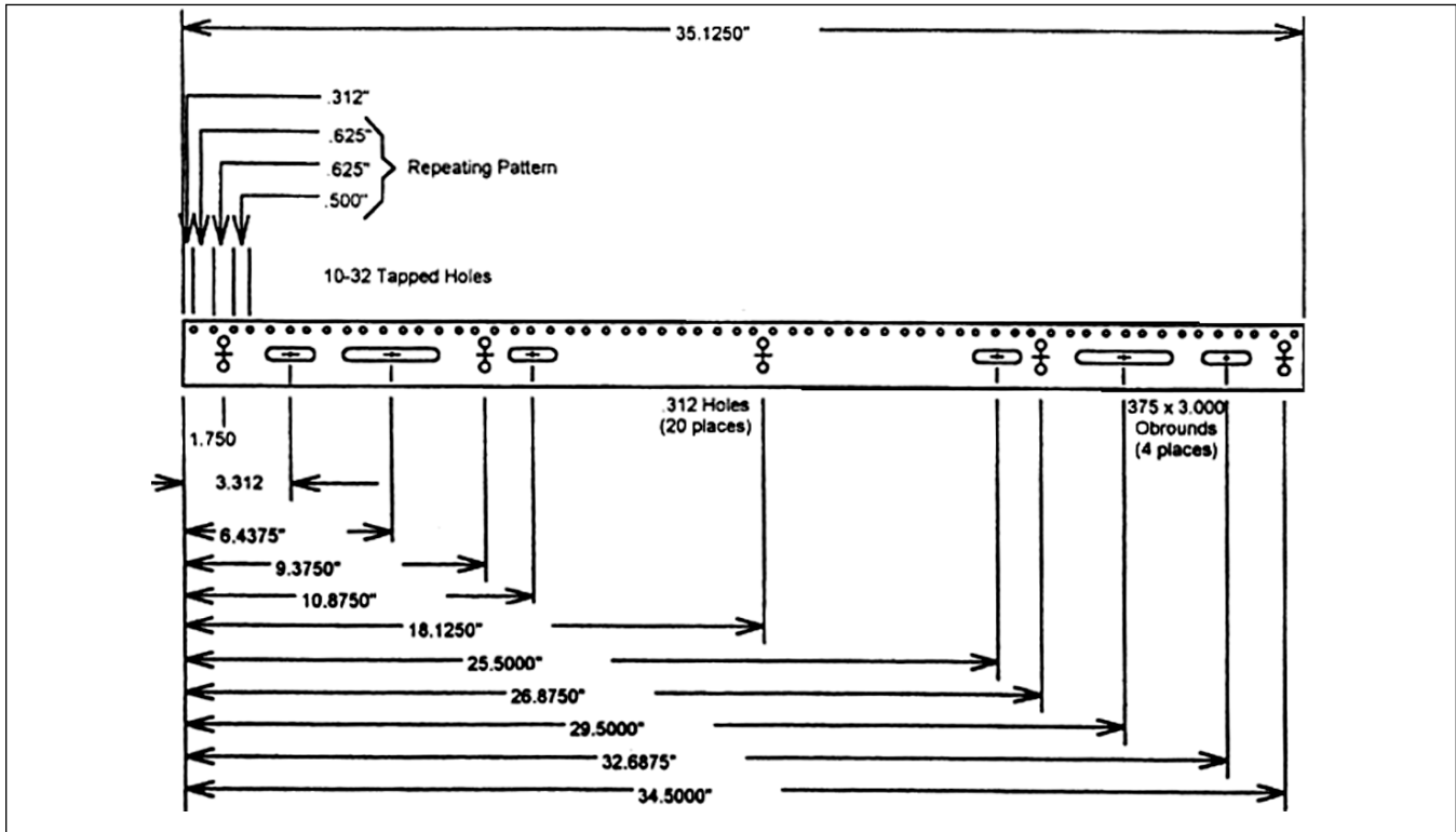
GBB Series Dimensions
