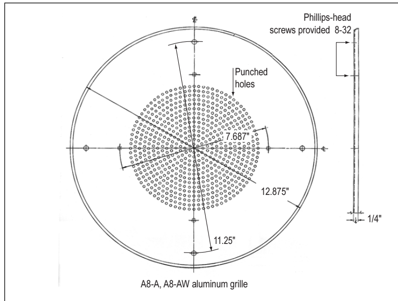
A8-A Aluminum Grille 8 screws, brushed alum. finish
