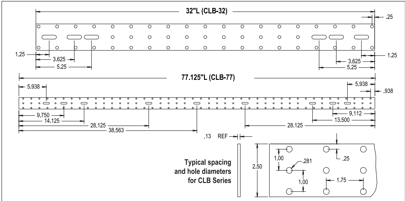
CLB Series Dimensions
