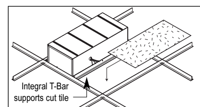
1' x 2' installation Replaces 1/2 of a 2' x 2' or 1/4 of a 2' x 4' ceiling tile. Integral T-Bar supports ceiling tile that was cut.
