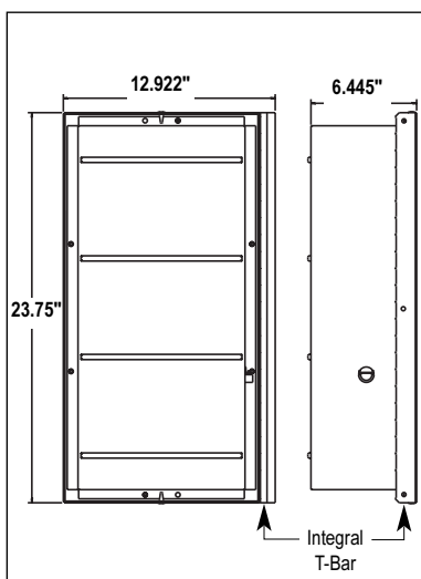
Dimensions LT Series 1' x 2' Systems with 0.8 cu.ft. backbox
