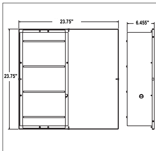
Dimensions LT Series 2' x 2' Systems with 0.8 cu.ft. backbox
