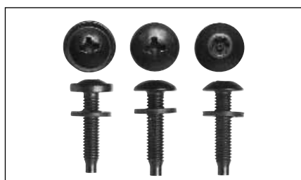
RSP RS RSV Phillips Phillips Torx® Finish Head Truss Head Star Post Head
