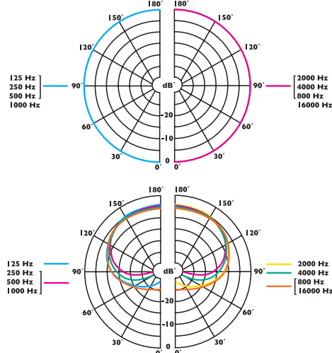
POLAR PATTERN
