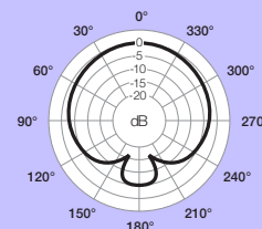
1 kHz Polar Response hypercardioid, measured at 6 inches
