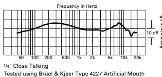
microphone frequency response: 40-20,000 Hz
