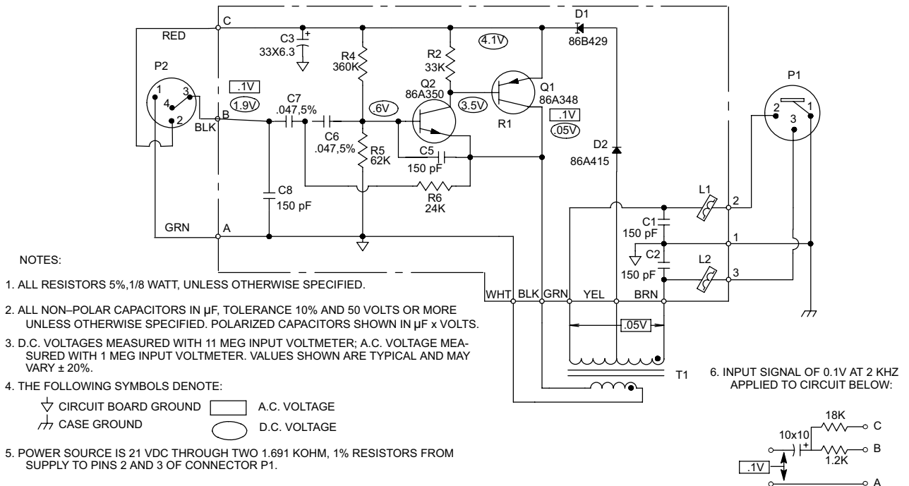
SM93 PREAMPLIFIER CIRCUIT DIAGRAM FIGURE 6
