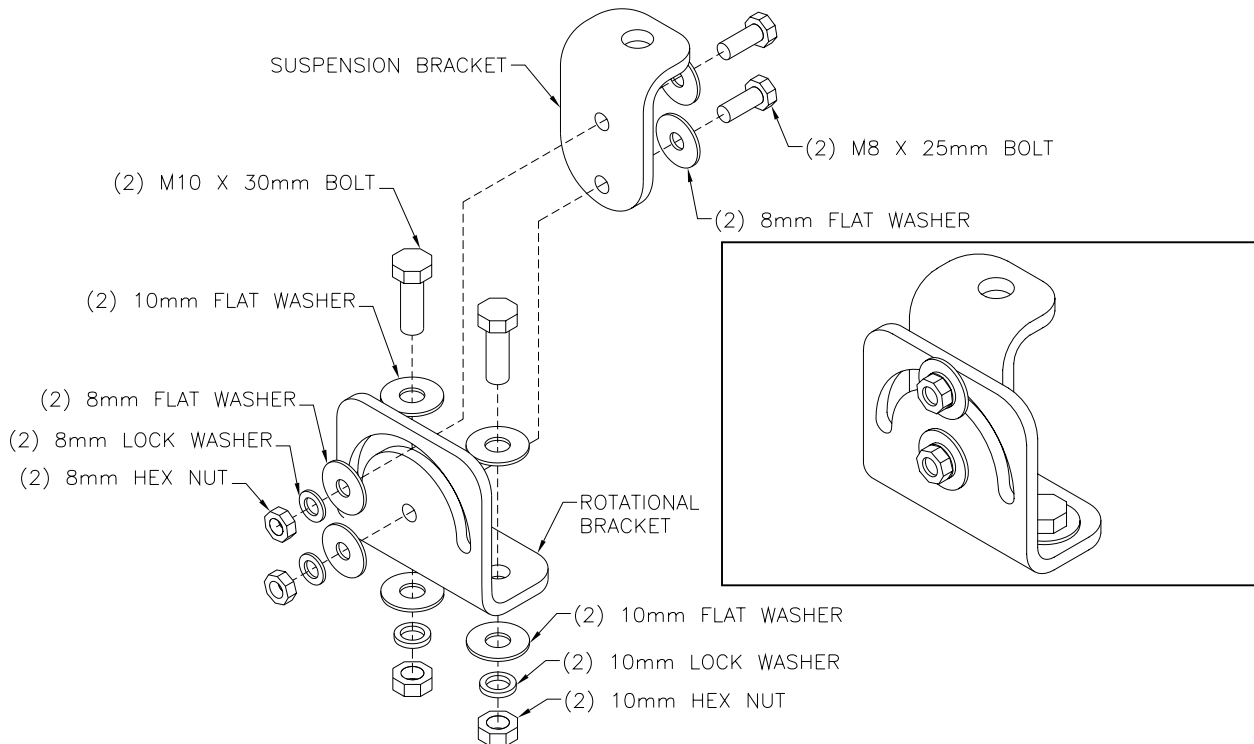
Figure 2: VB-TILT Assembly
